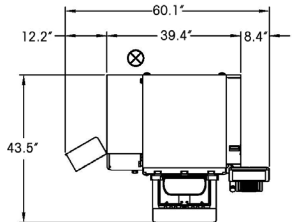
Dimensions in inches
